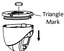
Figure 2-23 Disassemble the Camera
