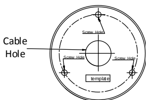
Figure 2-8 Drill Template
