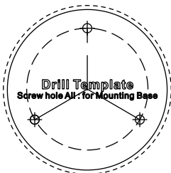
Figure 2-24 Drill Template
